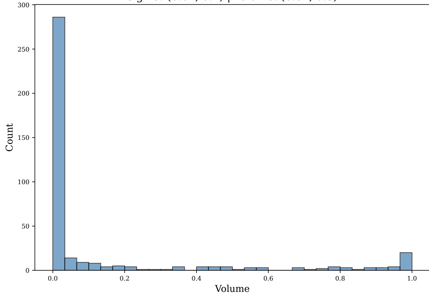
Volume Distribution of Downsampled Sequences (Filtered >20 seqs per motif) sigma: (0.02, 0.4) | volume: (0.07, 0.5)
